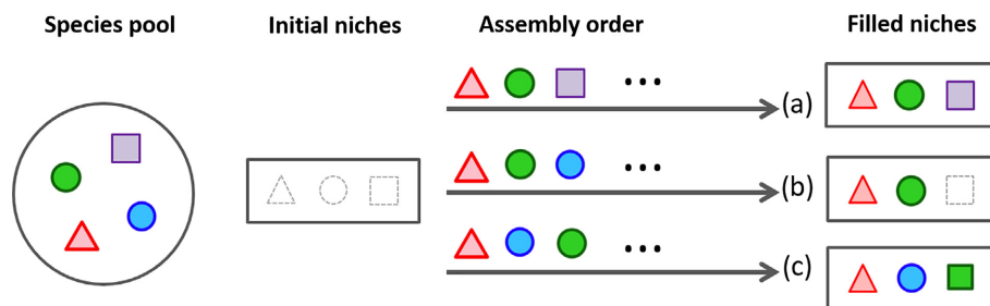
FIG. 1. Conceptual representation of mechanisms through which different ecological communities can be formed from the same species pool: (a) All species occupy independent niches. (b) An incumbent species blocks an ecologically similar species from joining the community through priority effects by niche incumbency (i.e., competitive exclusion). (c) An incumbent species blocks niche access to an ecologically similar species through priority effects, but ecological character displacement facilitates species coexistence and community assembly as each species utilizes independent ecological space. Symbol colors indicate different species. Symbol shapes denote the general ecological niche which that species occupies and dashed symbols represent vacant niches. Figure modified from Fukami (2015).
