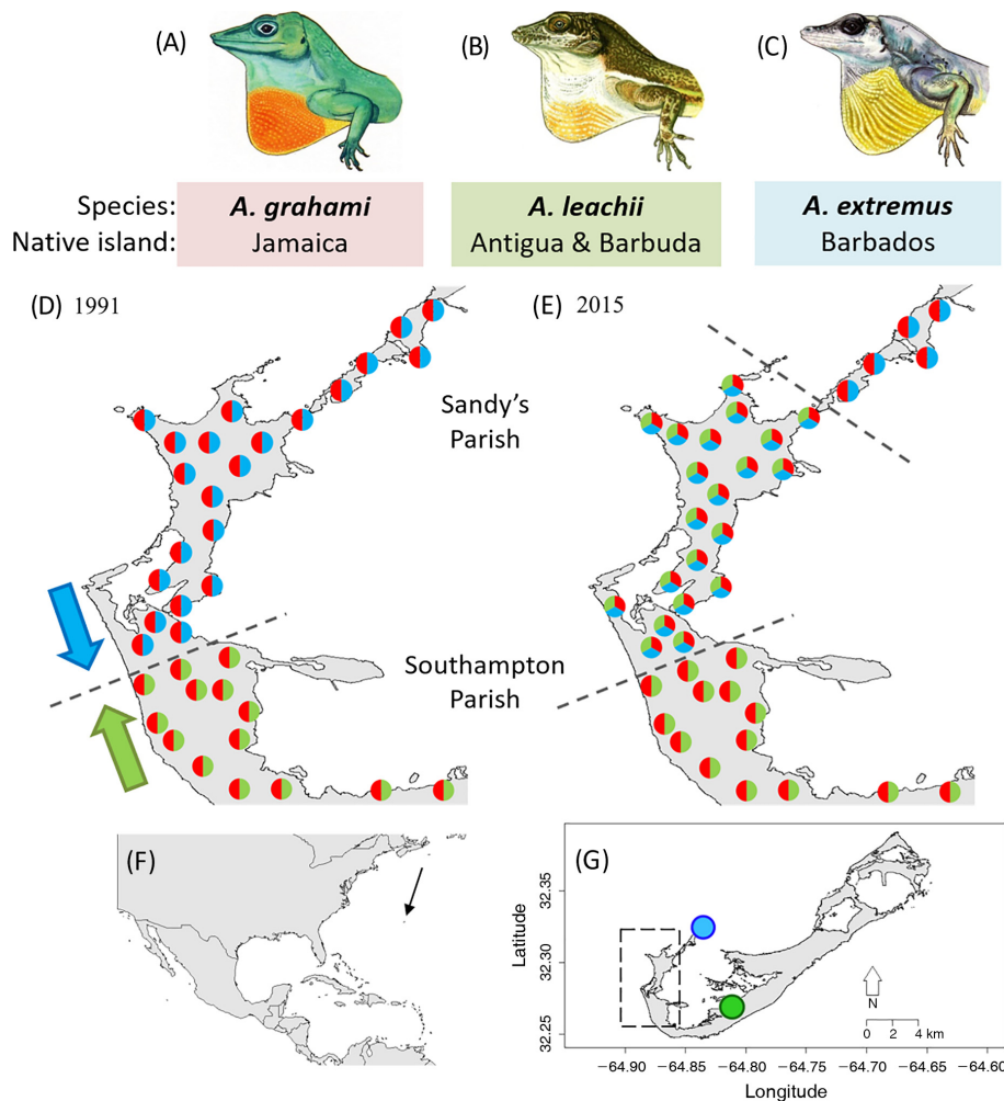
FIG. 2. Community assembly patterns at the contact zone between two species ([B] A. leachii ; green, and [C] A. extremus ; blue) which both underwent rapid directional dispersal from original geographically distinct locations on Bermuda (G). In 1964, only A. grahami (A; red) existed on Sandy's Parish, and was ubiquitous across the island except for the extreme northwestern tip where A. extremus established. By 1991, A. extremus had dispersed from its original site of introduction to form multiple two-species communities with A. grahami , and A. leachii had dispersed through Southampton Parish to the edge of the A. extremus range, creating a contact zone ([D]; dotted line, arrows represent direction of dispersal). In 2015 (E), A. leachii had invaded Sandy's Parish to form three species communities, but A. extremus had failed to invade through the original contact zone with A. leachii in Southampton Parish. Native islands from which each species originated are indicated under (A)–(C). The geographic location of Bermuda is shown in (F). Dashed lines represent range edges. Anole illustrations are used with permission from Schwartz and Henderson (1985).
