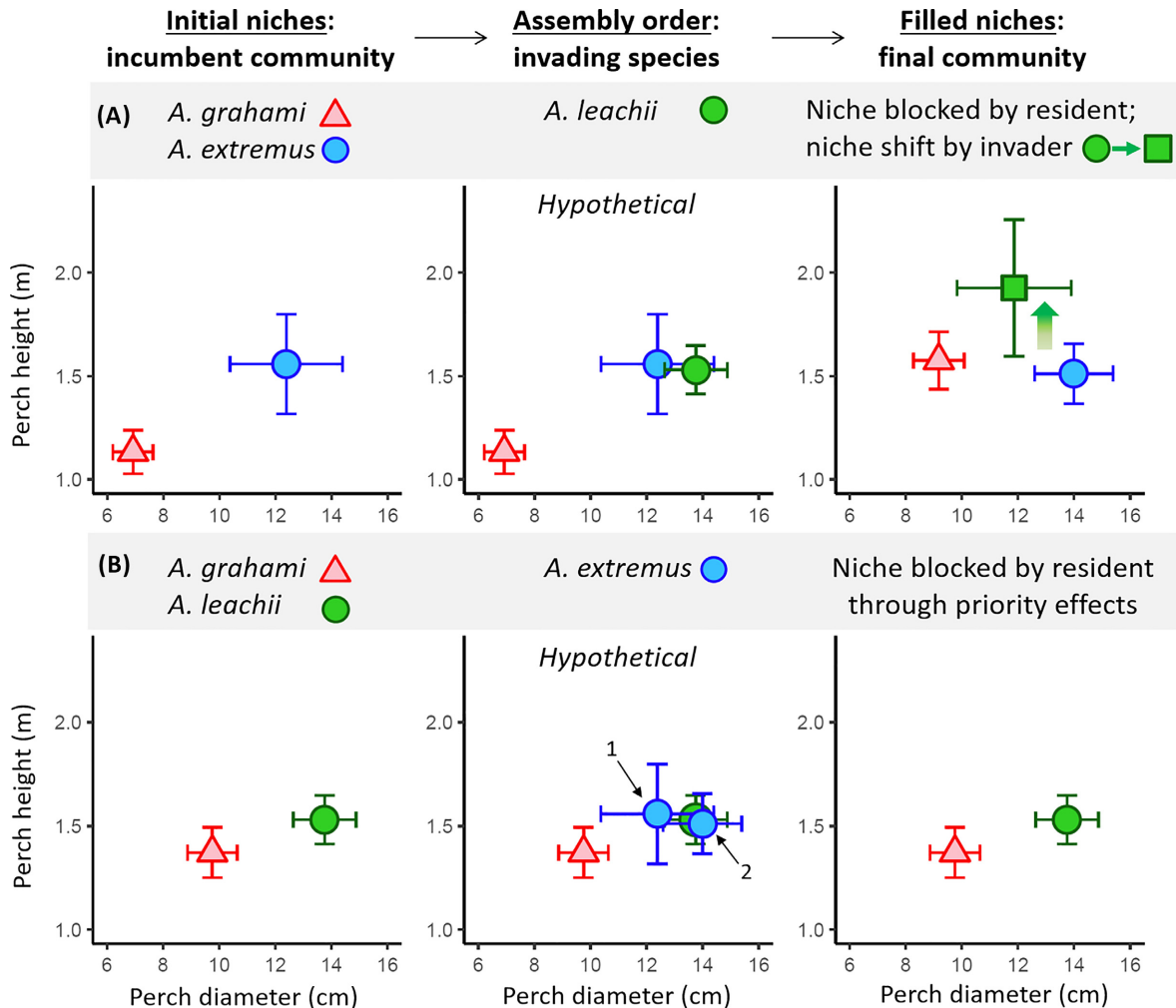
FIG. 3. Community assembly and ecological niche organization of nonnative Anolis lizards in Bermuda. Plots represent ecological niches of each species, here described through the axes along which divergence most commonly occurred to facilitate coexistence; structural habitat use (points represent species mean \pm 1 SE). (A) Anolis extremus blocks ecological access to A. leachii attempting to join grahami-extremus communities through priority effects and niche incumbency. However, A. leachii responds by shifting its niche into unoccupied ecological space (i.e., assembly mechanism shown in Fig. 1c). (B) However, A. extremus is unsuccessful in invading grahami-leachii communities (either before [1] or after [2] the invasion of A. leachii ) as priority effects from A. leachii block access to the preferred ecological space of A. extremus (i.e., assembly mechanism shown in Fig. 1b). The invading species (in both [A] and [B]) always significantly overlaps with the incumbent species in both axes of ecological space. As in Fig. 1, different species are denoted by colors and different niches by shapes.
